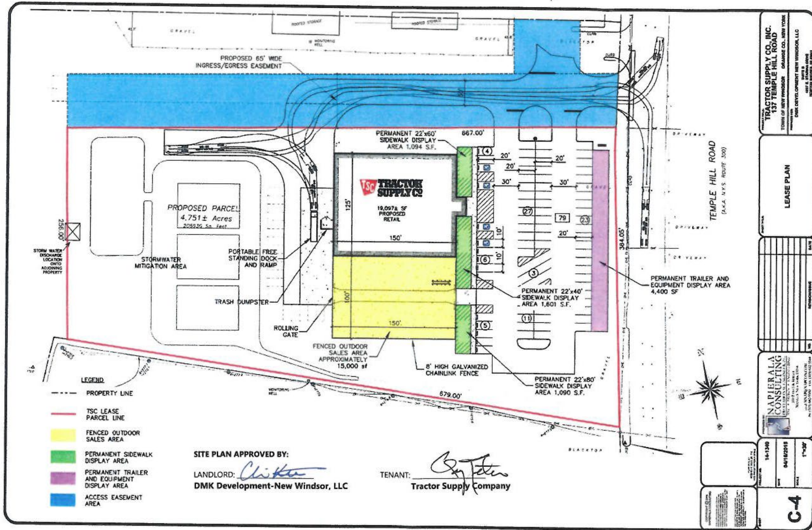
EXHIBIT "C" PRELIMINARY SITE PLAN
